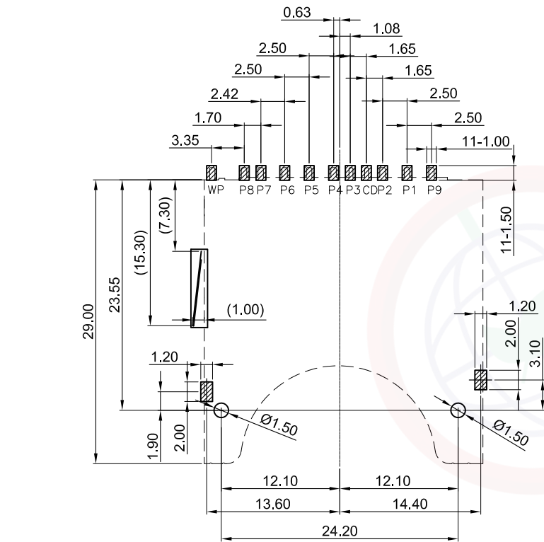
RECOMMEND PCB LAYOUT (TOLERANCE=±0.05)
